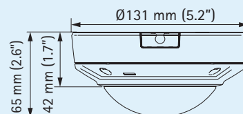
AXIS M3007-PV
