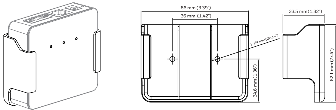
Base Bracket
